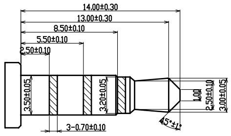
PLUG SPEC
