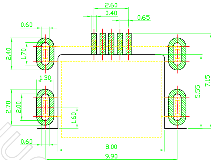
RECOMMEND PCB LAYOUT GENERAL TOLERANCE ±0.05
