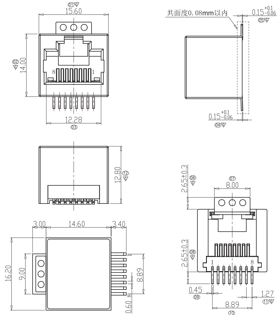
PCB LAYOUT/TOP VIEW TOLERANCE=±0.05
